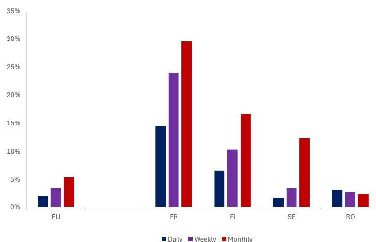
Figure 4 – Contribution of nuclear energy to daily, weekly, and monthly flexibility needs in energy volume in the EU and selected Member States in 2030.
