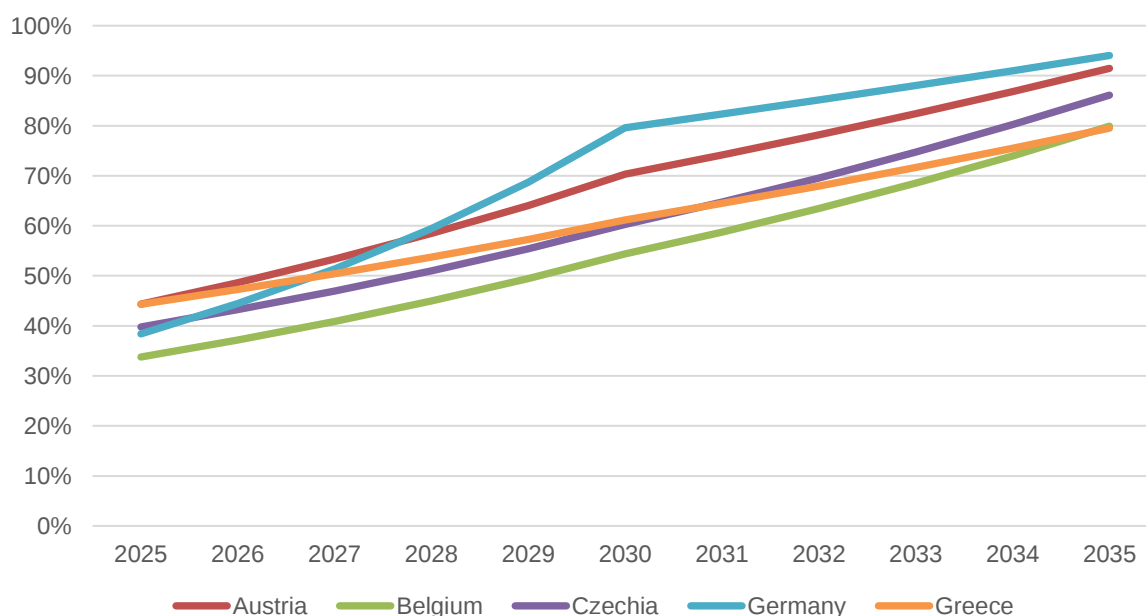
Figure 17: Estimated FTTH coverage (excl. FTTB) in Austria, Belgium, Czechia, Germany and Greece in 2035 under the status quo (in % of HH)
